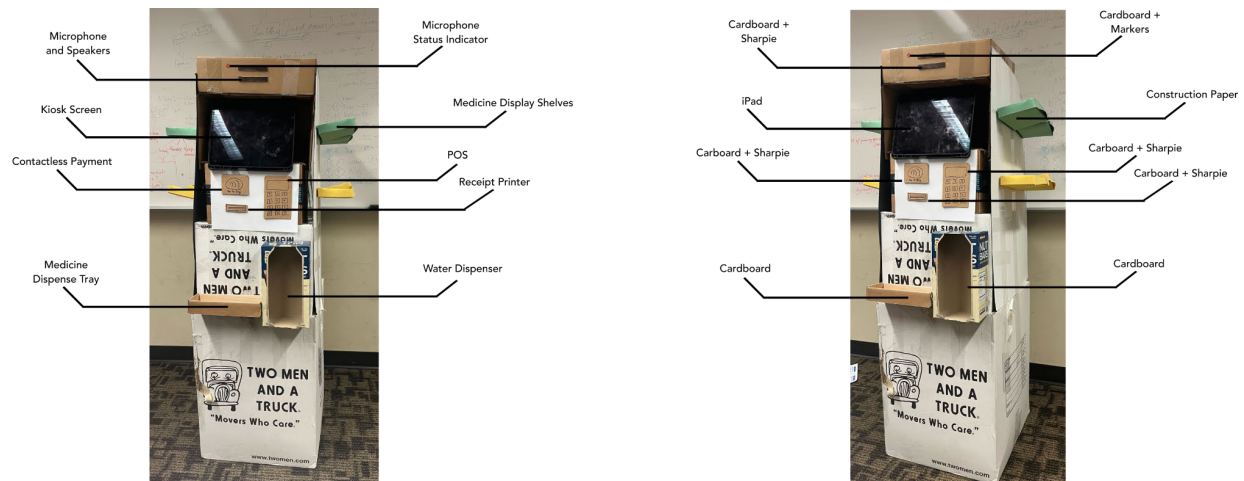
Figure 2. Components and materials used to build the kiosk prototype.
